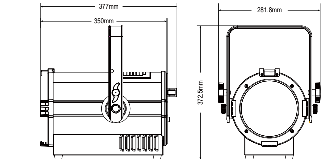
Maximum Spot - 55°
