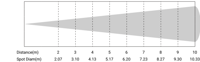
Maximum Spot - 55°
