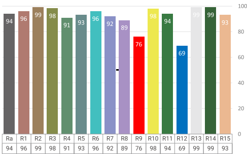
Minimum Spot - 15°
