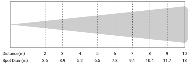
Max. Spot - 60°
