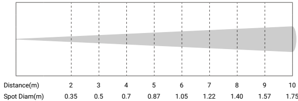
Minimum Spot - 10°
